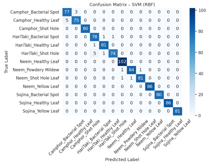
Fig. 2. Confusion matrix on the test set using an SVM classifier trained on DINOv2 features.
