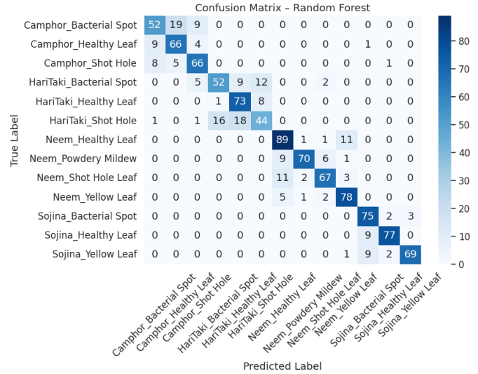
Fig. 22. Confusion matrix on the test set using an Random Forest classifier trained on SimCLR features.
