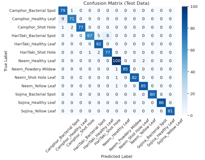
Fig. 1. Confusion matrix on the test set using an MLP classifier trained on DINOv2 features.
